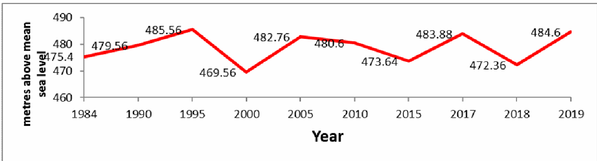
Fig. 5: Water level fluctuation of Darbandikhan during 1984-2017.
