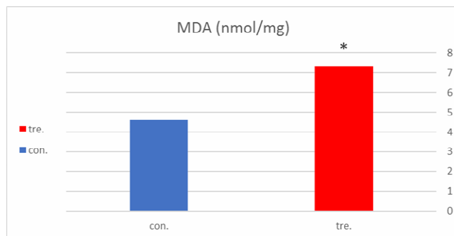
Fig. 2 : MDA level of control and treated groups at p \leq 0.05 . *indicate a difference significantly between control and treatment groups.
